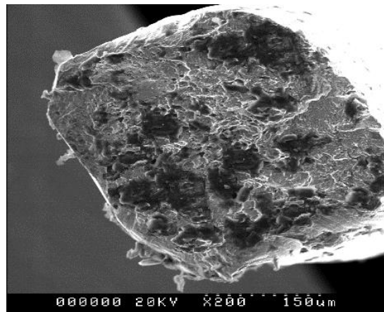
Figure 5. The microstructure of the VT1-0 implant fracture.
