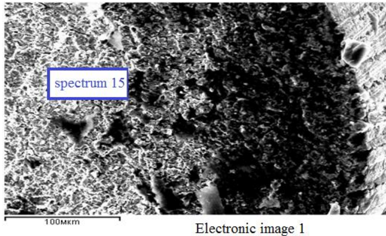
Figure 4. The microstructure of the NiTi implant fracture.
