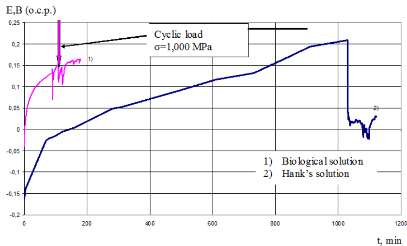
Figure 3. The dependence of the open-circuit potential of the implant surface (VT1-0) on the exposure time in biological solutions at a temperature of 37 °C and when exposed to load.
