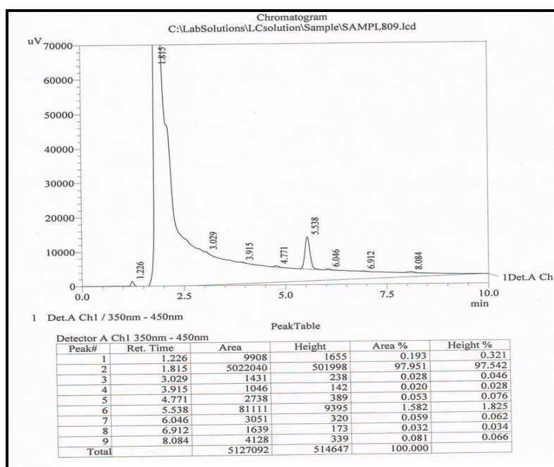
Figure 3: Chromatogram of Control Reduced Glutathione
