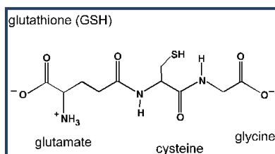
Figure 1: Chemical structure of glutathione
