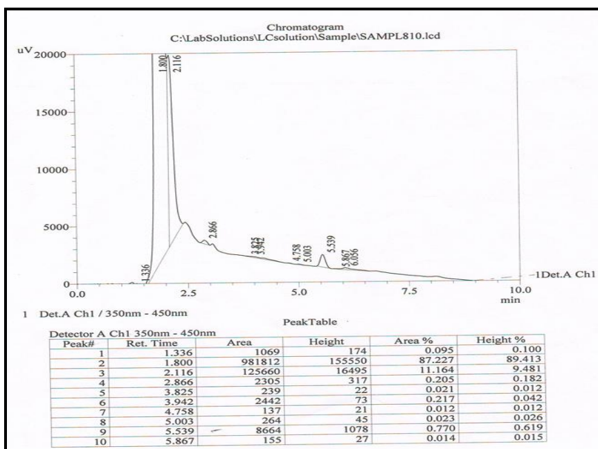
Figure 4: Chromatogram of Reduced Glutathione for (Renal stone Sample)
