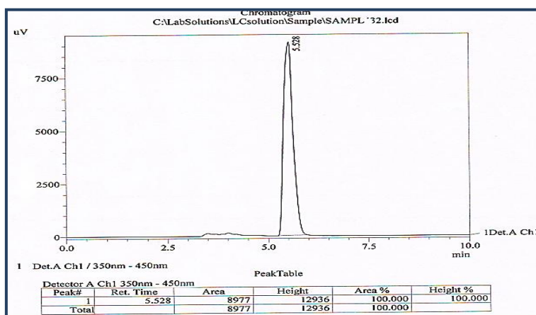
Figure 2: Standard Curve of Reduced Glutathione
