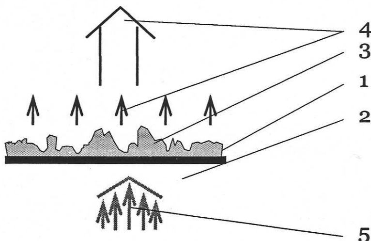
1 – heat exchanger; 2 – heater; 3 – organic matter (manure); 4 – the mass of water vapor; 5 – heat flux Figure 1: Flow chart of drying organic waste
