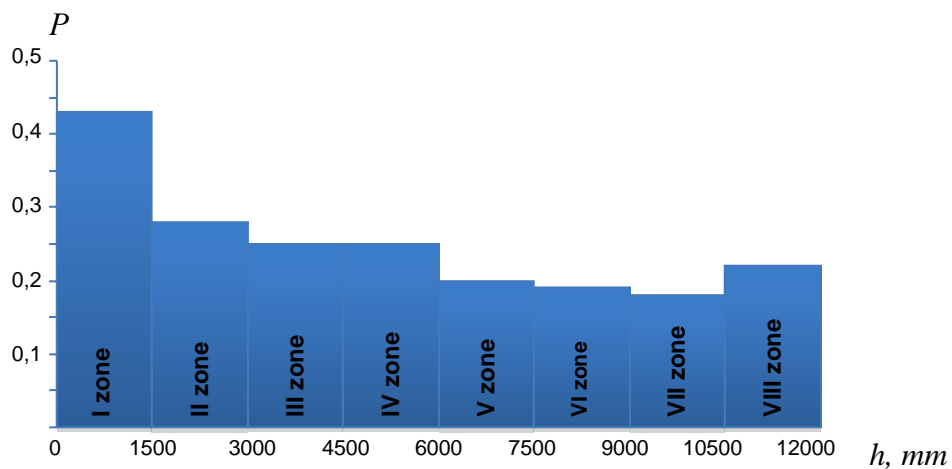
Fig 3: The dependence of the probability of occurrence of unacceptable deviations on shell height.
