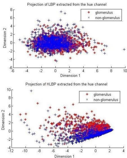
Fig. 2. Texture descriptor LBP_{8,1}^{riu} and HLBP_{8,1}^{36,riu} in the hue channel are projected into 2-dimensional subspaces by PCA to visualize their discriminative powers. In the figure, a red * represents a glomerulus patch, and a blue x corresponds to a non-glomerulus image.
