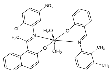
Figure 4: The metal-ligand ternary binding proposed structure.
