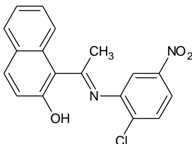
Figure 2: Secondary ligand 1-[(1E)-N-(2-chloro-5-nitrophenyl)ethanimidoyl]naphthalen-2-ol
