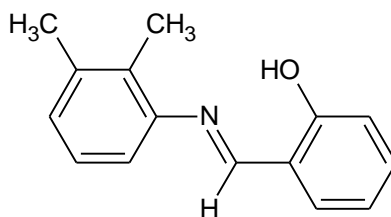
Figure 1: Primary ligand 2-((E)-[(2,3-dimethylphenyl)imino]methyl}phenol
