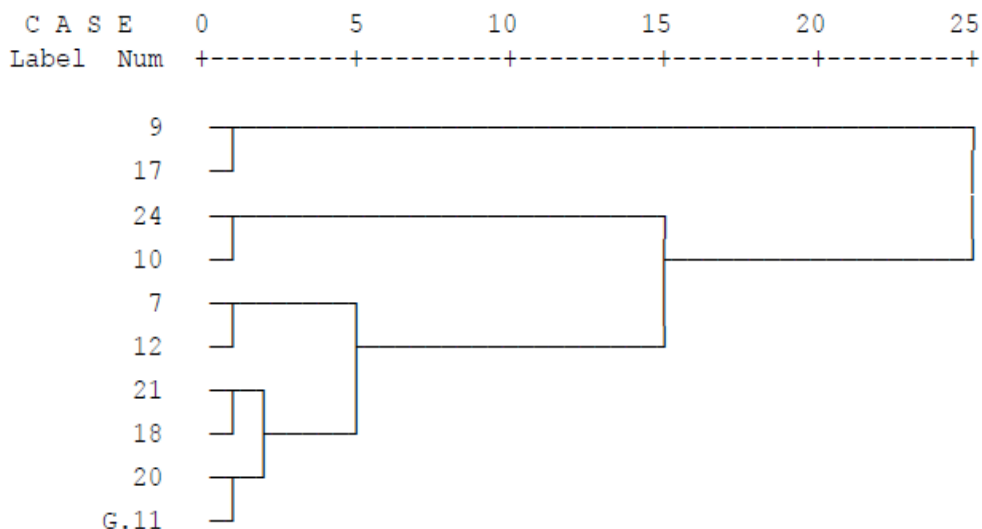
Fig.3: Cluster diagram for 10 wheat genotypes classified by Viscoamylograph parameters for whole meal (100%) extraction rate under normal conditions (N).
