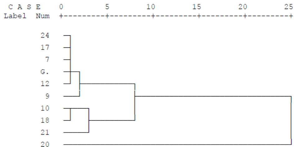
Fig.1: Cluster diagram for 10 wheat genotypes on basis of agronomic traits under normal conditions (N).
