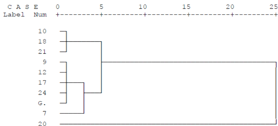
Fig.2: Cluster diagram for 10 wheat genotypes on basis of agronomic traits under drought conditions (D).
