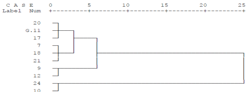
Fig.4: Cluster diagram for 10 wheat genotypes classified by Viscoamylograph parameters for whole meal (100%) extraction rate under drought conditions (D).
