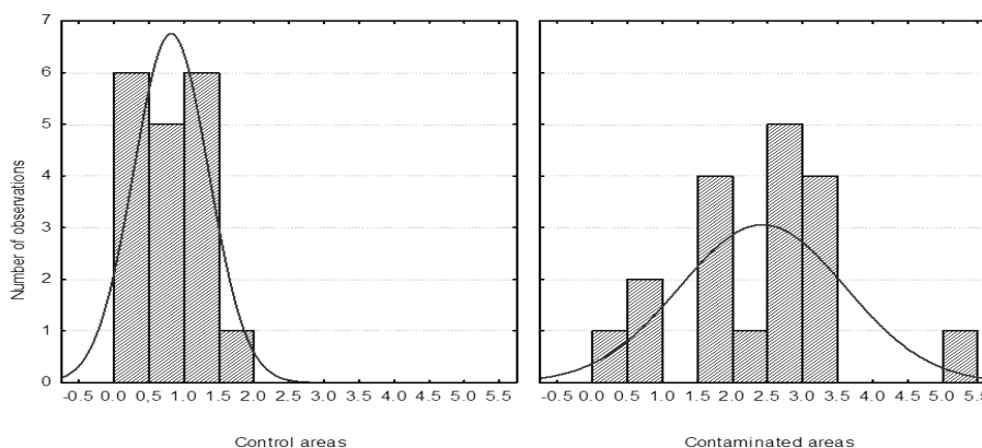
Figure 2: Histogram of lead concentrations in bees from control and contaminated areas
