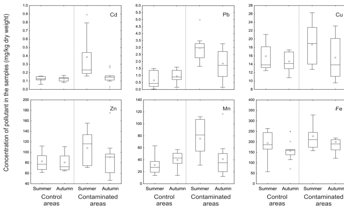
Figure 3: Box plots of concentration data for six heavy metals in the bodies of bees in contaminated and control environments in two seasons. Full range of variation (between minimum and maximum non-outliers whiskers), the likely range of variation (the IQR; box), outliers (open circles), extremes (asterisks), median (horizontal line), and mean (open square within box)
