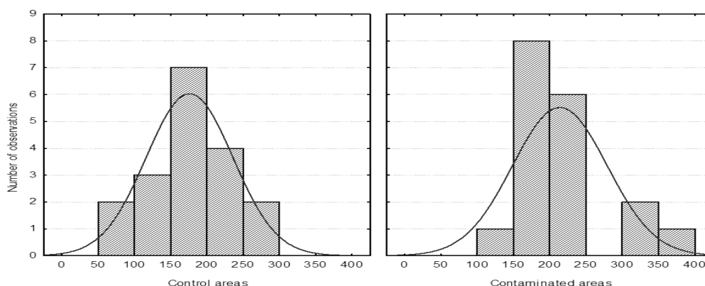
Figure 1: Histogram of iron concentrations in bees from control and contaminated areas
