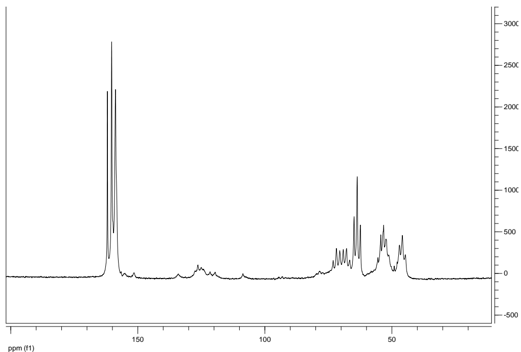
Figure 2: NMR-spectroscopy of modified by \alpha -naphthol of UFR-oligomers on nuclei of carbon atom ^{13}\text{C}
