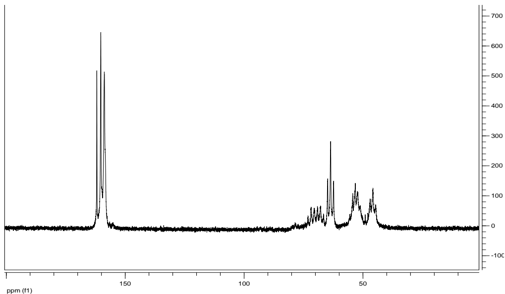
Figure 1: NMR-spectroscopy of UFR on nuclei of carbon atom ^{13}\text{C}
